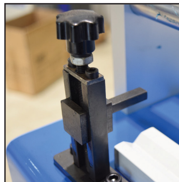
Rebar Sample Clamping
