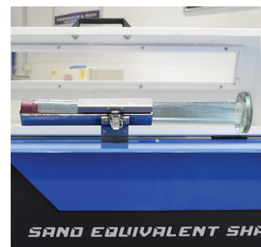
Single Cylinder
